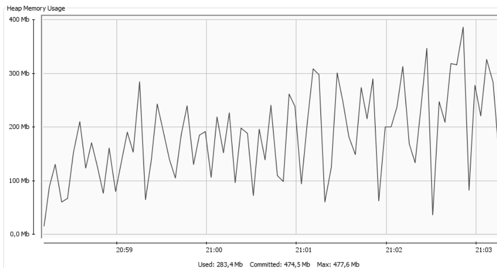
Figure 7 Memory heap utilization
