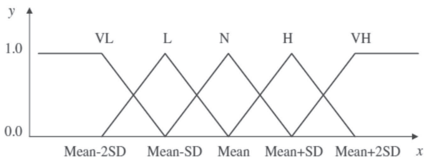
Figure 1. Membership function
